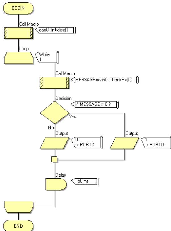
Figure 7.2 Receive signal flowchart
