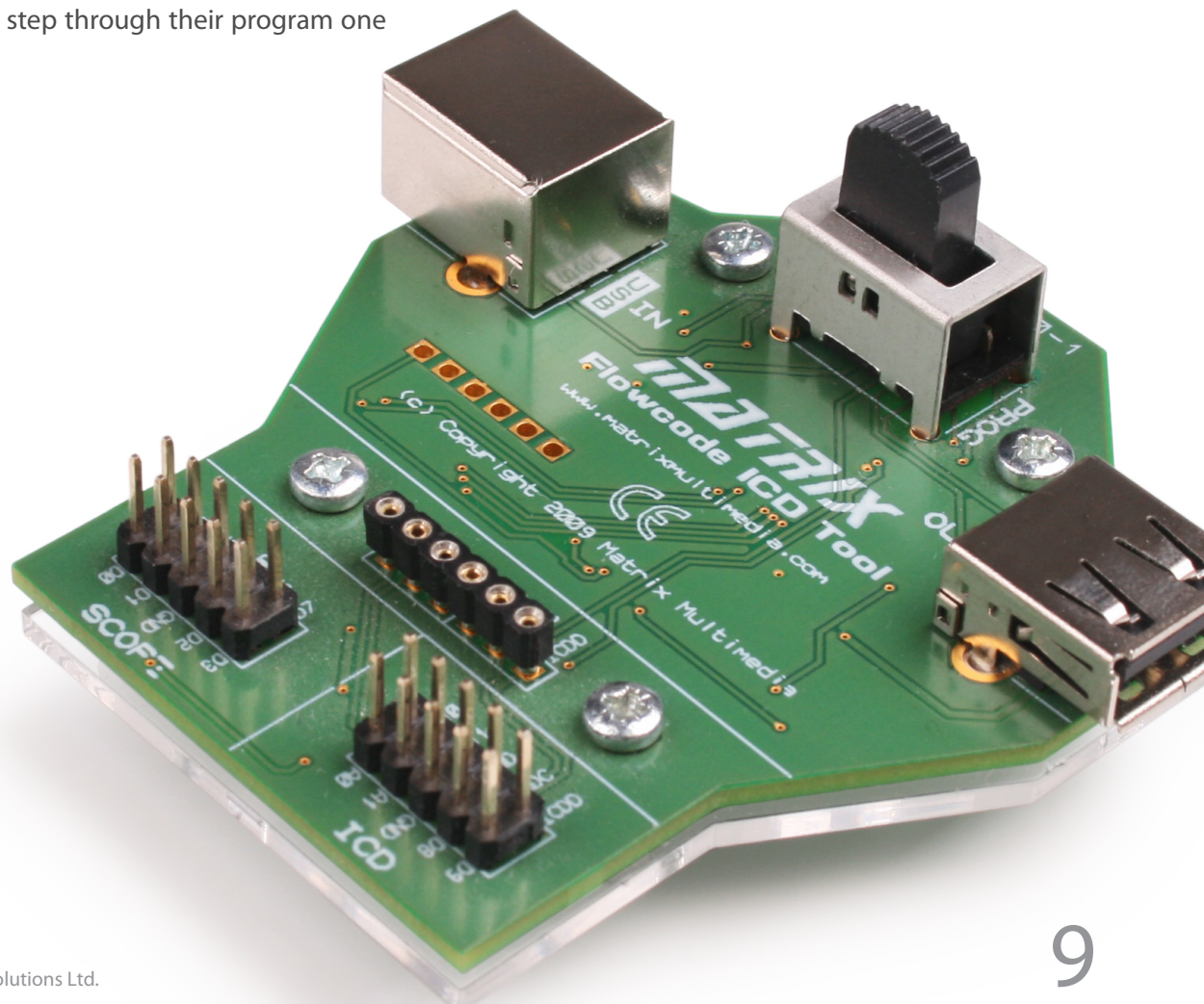
Using FlowKit with ECIO and E-blocks adaptor board
